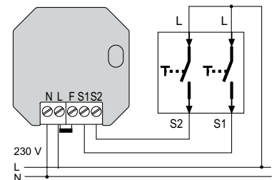
Switch connection S1, S2: ON/OFF
